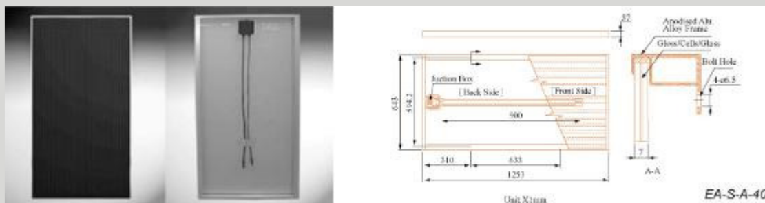
amorphous silicon pv module
